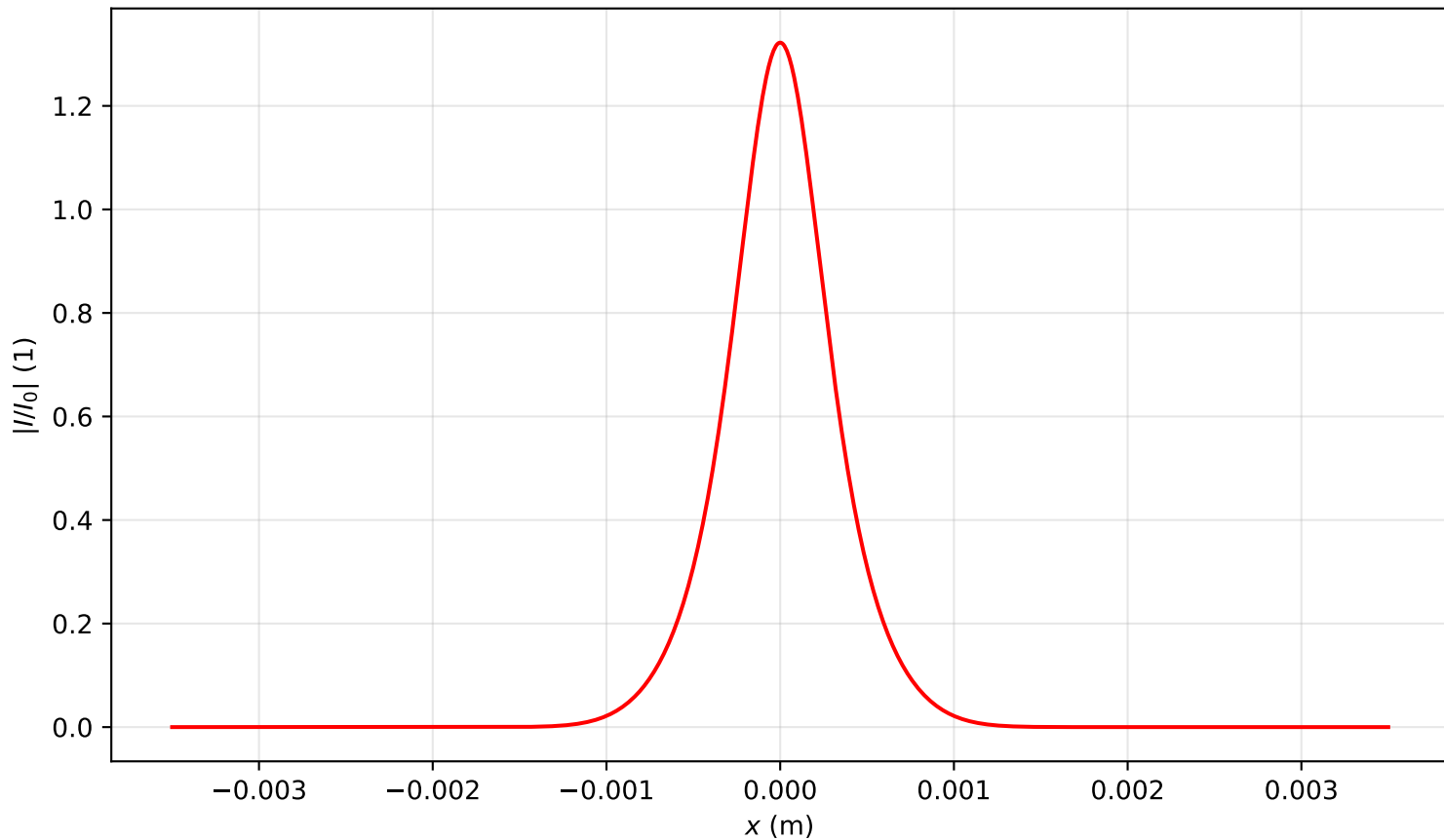
Intensity profile I(x, y = 0, z = 0.716)/I_0 , P_{in}=1.0P_{cr} , artificial time
